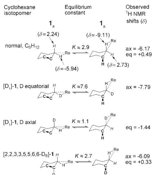
Scheme 2. Equilibria between axially and equatorially complexed species for various isotopomers with midrange-fitted empirical equilibrium constants. All equilibria are in fast exchange on the NMR timescale at the temperatures employed resulting in only weighted-averaged shifts being observed. In each case one of the two (equivalent) bonds antiperiplanar to the complexed bond is shown in bold. Chemical shifts in brackets are estimated values based on empirical data for each proton that would be observed if no exchange were occurring.
