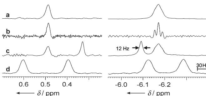
Figure 1. Signals due to the protons of a bound methylene unit in a, b) [\text{CpRe}(\text{CO})_2(\text{cyclohexane})] ( 1 ), c) a mixture of 1 and [\text{CpRe}(\text{CO})_2([2,2,3,3,5,5,6,6\text{-D}_8]\text{cyclohexane-}\eta^2\text{-C}^1\text{H}_2)] ( [\text{D}_8]\text{-1} ), and d) [\text{CpRe}(\text{CO})_2([^{13}\text{C}_6]\text{cyclohexane})] ( [\text{C}_6]\text{-1} ) in their ^1\text{H} NMR spectra at 173 K. [5] The spectra in (a), (c), and (d) have line broadening of 5 Hz and the spectrum in (b) is resolution-enhanced with Gaussian multiplication. All spectra shown were obtained for 8:82:10 [\text{D}_{12}]\text{pentane/isobutene/cyclohexane} solvent mixtures.
